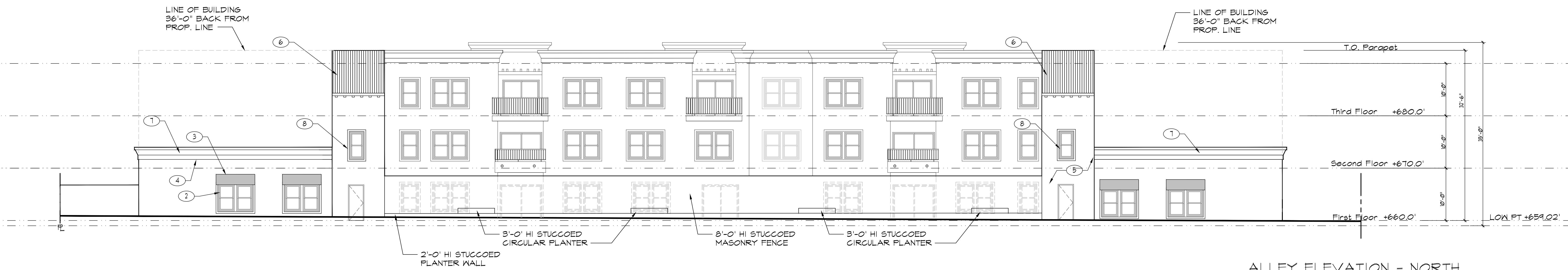
ALLEY ELEVATION - NORTH SCALE 1/8"=1'-0"
